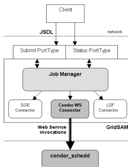
Figure 3: GridSAM architecture
