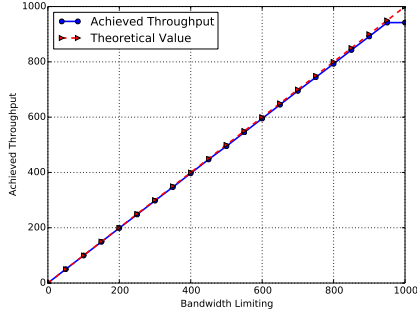
Fig. 11: Achieved throughput by Open vSwitch after bandwidth limiting
