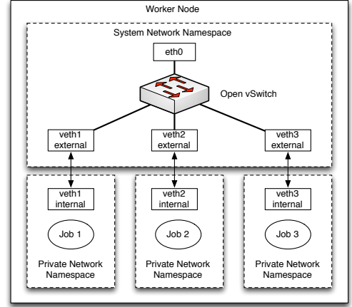
Fig. 2: Open vSwitch bridging configuration for different batch jobs. (Each dotted square represents a separate network namespace)
